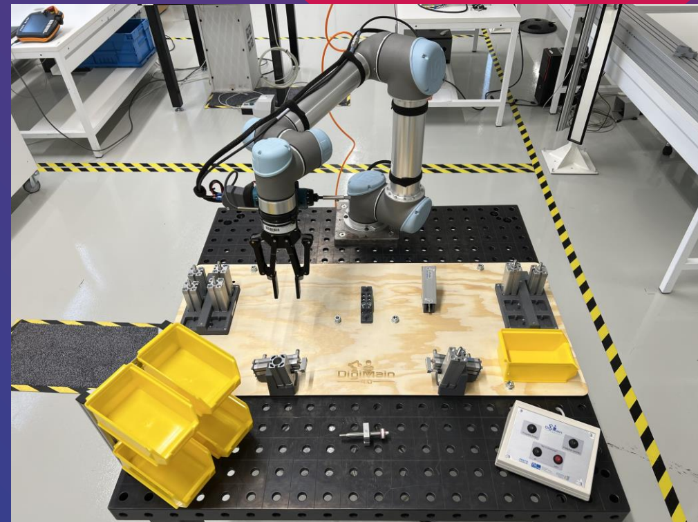
Cobot Demonstrator
