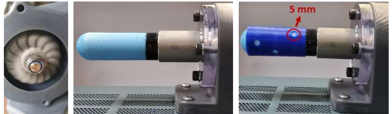
Turbine system silencer with and without a 'cover'
